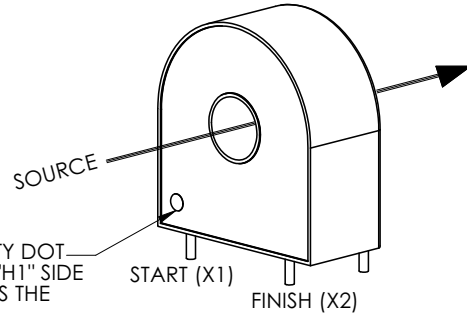
CR8300 Series Current Transformers
